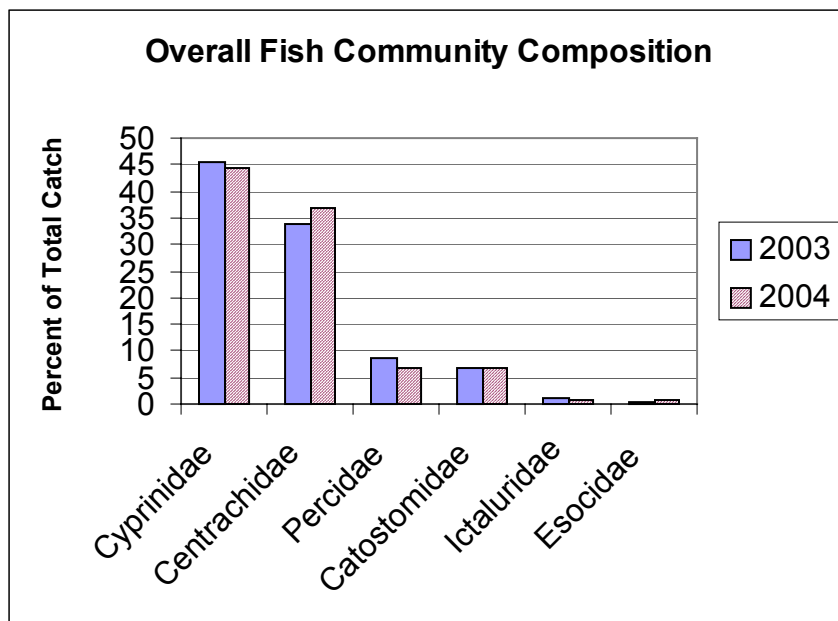
Figure 2. Overall fish community composition for 2003 and 2004.
